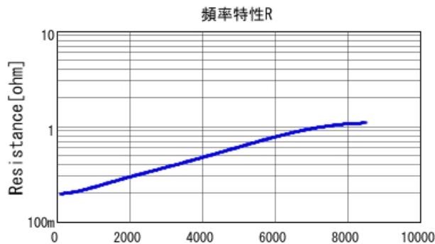
GCM0335C1E100FA16 R DCOV, 25degC
