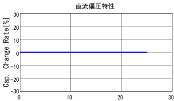
GCM0335C1E100FA16 C-DC bias capchange, 25.0degC, A
