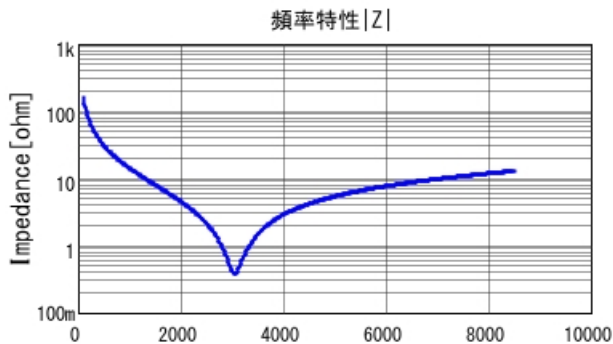
GRT0335C1E100FA02 |Z| DCOV, 25degC
